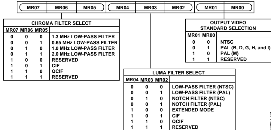
Figure 38. Mode Register 0
